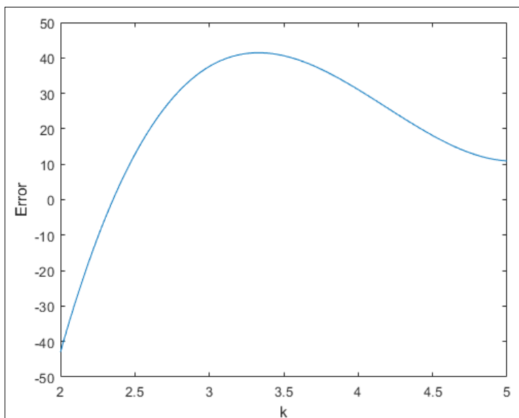
Fig 4: A plot of the error versus the number of points for Gauss Quadrature – Function 2
