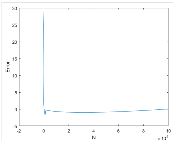
Fig 1: A plot of the error versus the number of samples for Monte Carlo – Function 1
