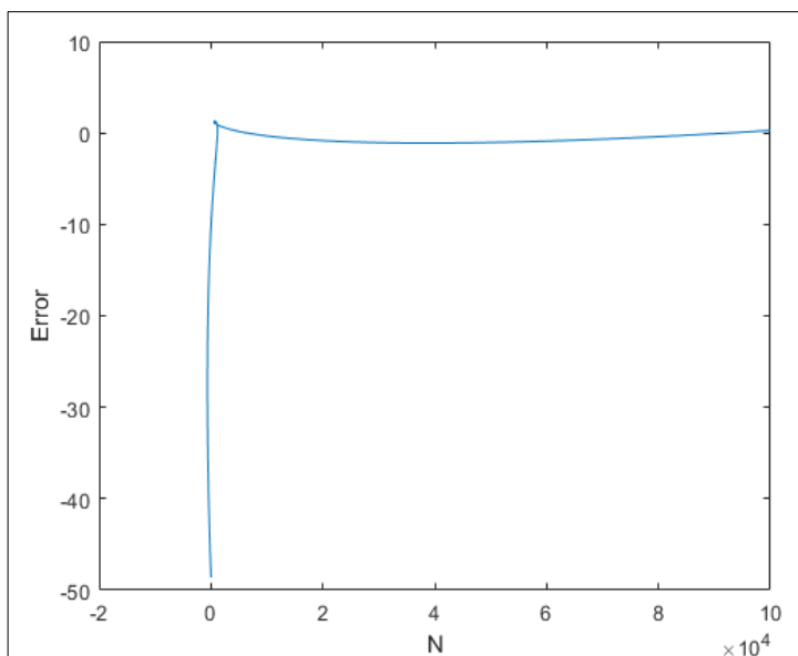
Fig 2: A plot of the error versus the number of samples for Monte Carlo – Function 2
