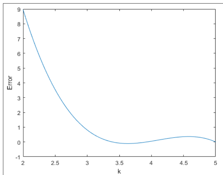
Fig 3: A plot of the error versus the number of points for Gauss Quadrature – Function 1
